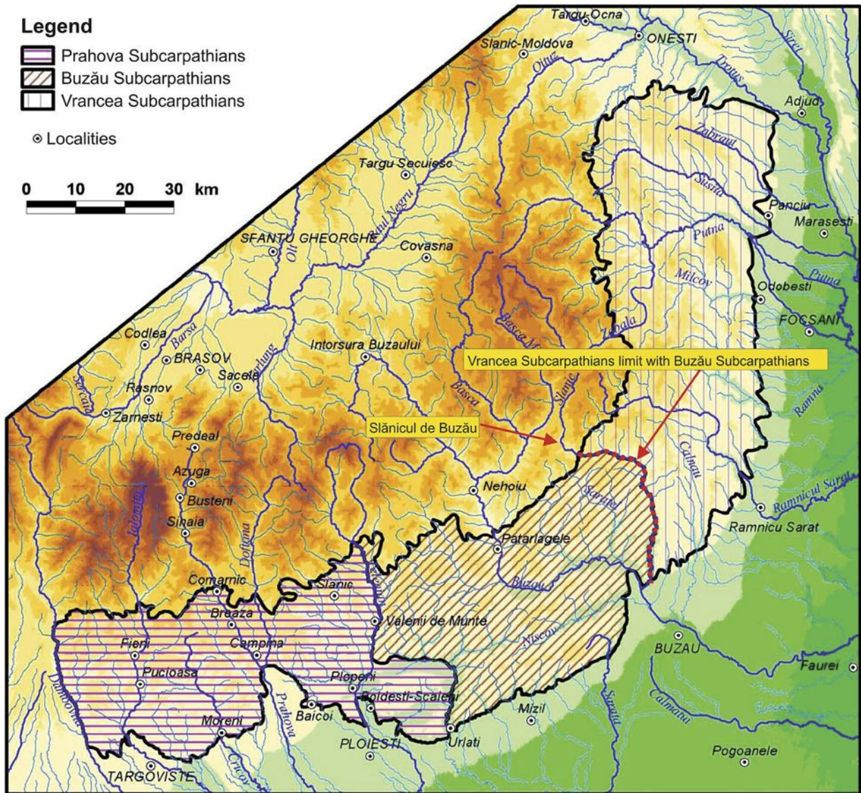
Fig. 1. Location of Slănicul de Buzău Valley in-between the Buzău and Vrancea Subcarpathians (after Chendeş, 2011).
